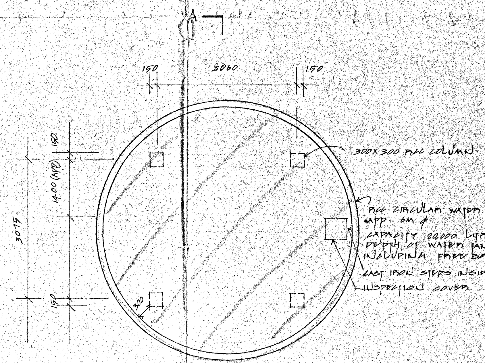
PLAN AT WATER TANK LVL.
